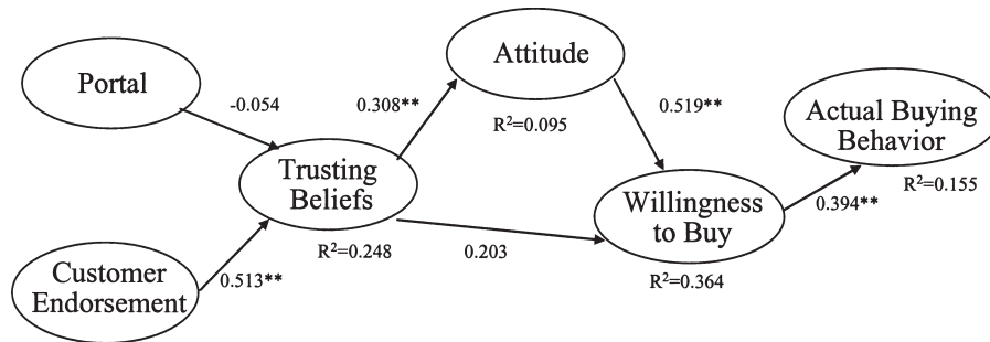
Figure 5. Path Estimate (Standard Error) of PLS Analysis ** significant at the 5 percent level.
